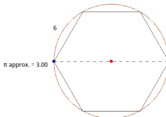
Figure 8.12: Hexagone régulier inscrit
