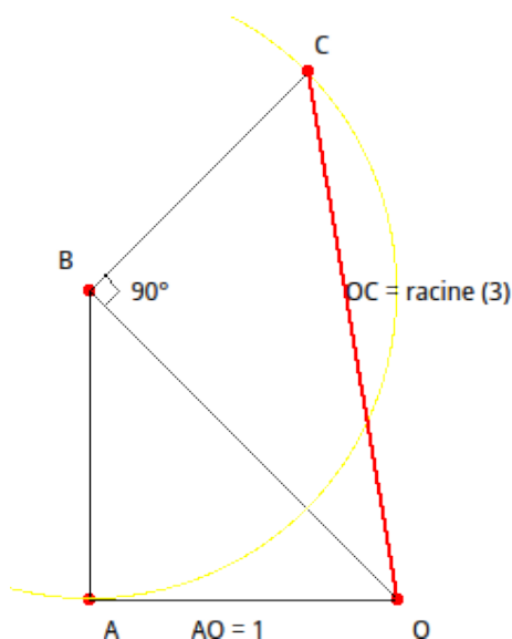
Figure 8.7: Construction de la racine 3
