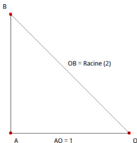
Figure 8.6: Construction de la racine de 2
