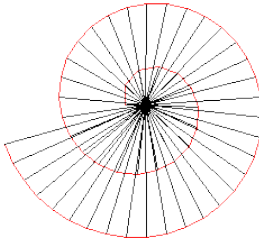
Figure 8.8: Spirale de Teodoro
