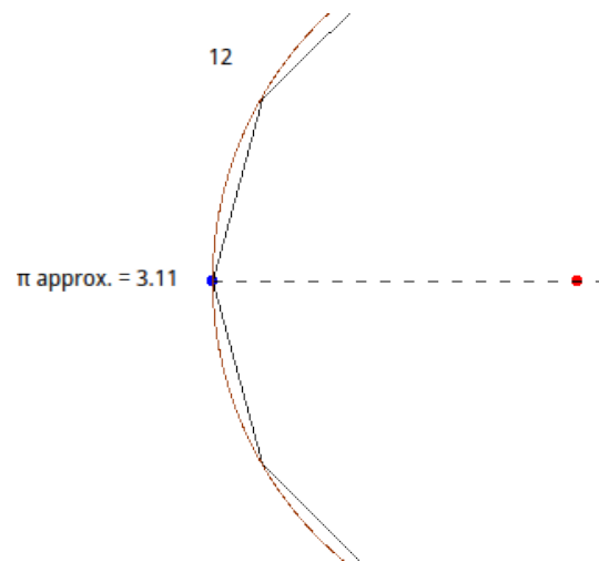
Figure 8.13: Approximation de PI
